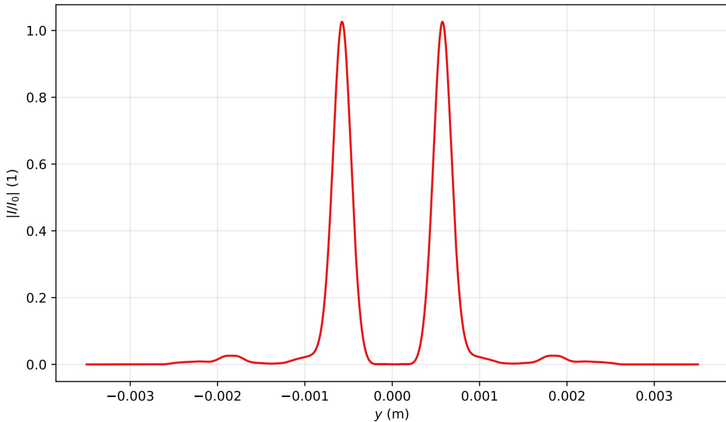
Intensity profile I(x=0, y, z=1.672)/I_0 , \text{Pin}=8.0\text{Pcr} , artificial time
